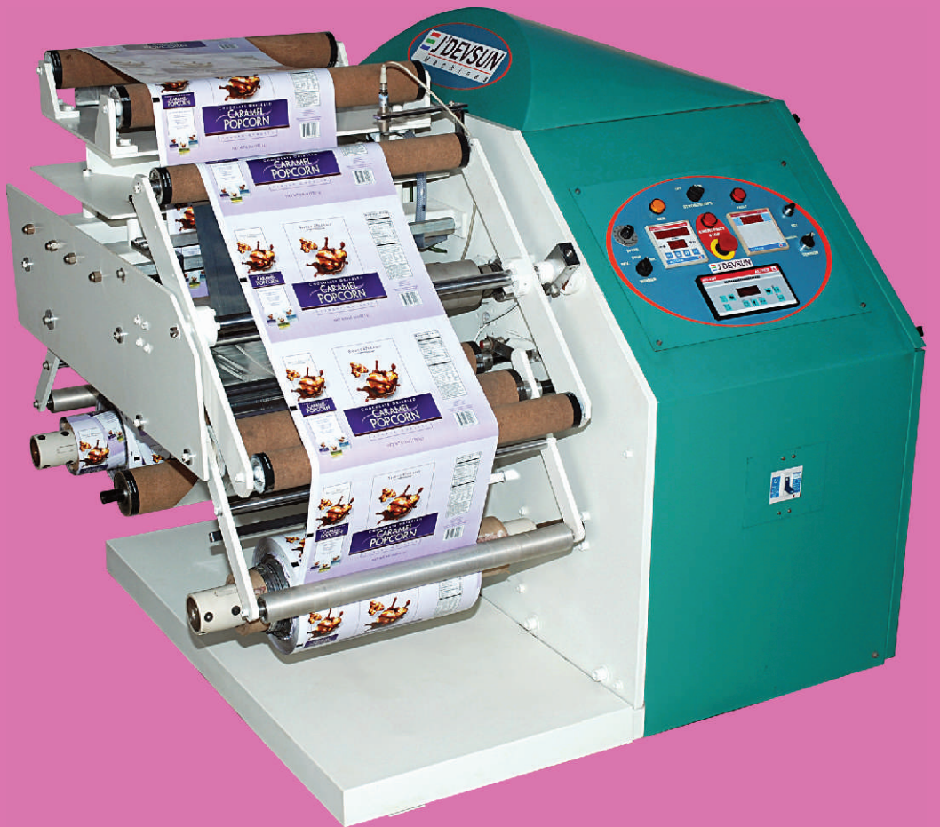
Doctoring Machine
